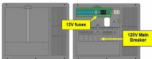
Load Center Panel w/120 volt Main Breaker
