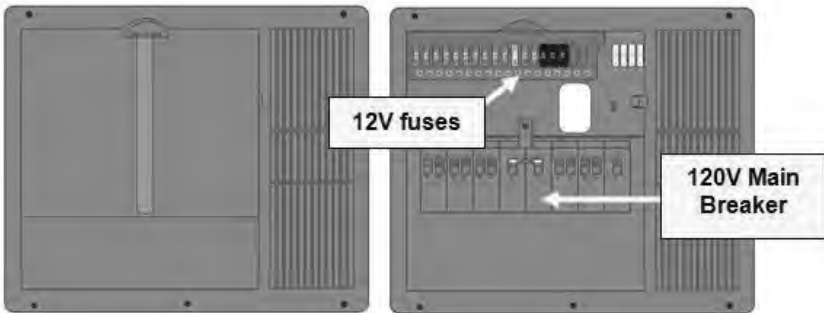
Typical Load Center Exterior Panel
