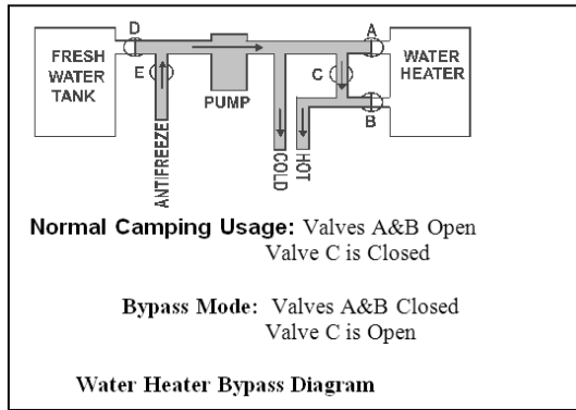
Factory installed water heater bypass
