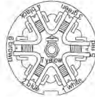
7-way trailer plug Car end, rear view
