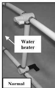
Two Valve Water Heater Bypass
