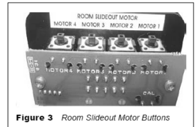
Figure 3 Room Slideout Motor Buttons
