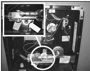
Water heater drain plug location
