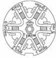
7-way trailer plug-rear view
