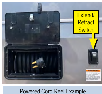
Powered Cord Reel Example
