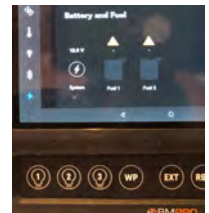
BMPro Example
