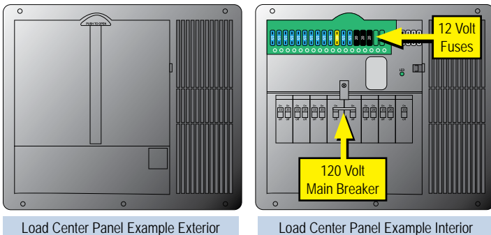
Load Center Panel Example Exterior
