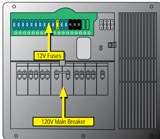
Load Center Panel w. 120 Volt Main Breaker
