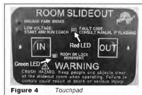
Figure 4 Touchpad
